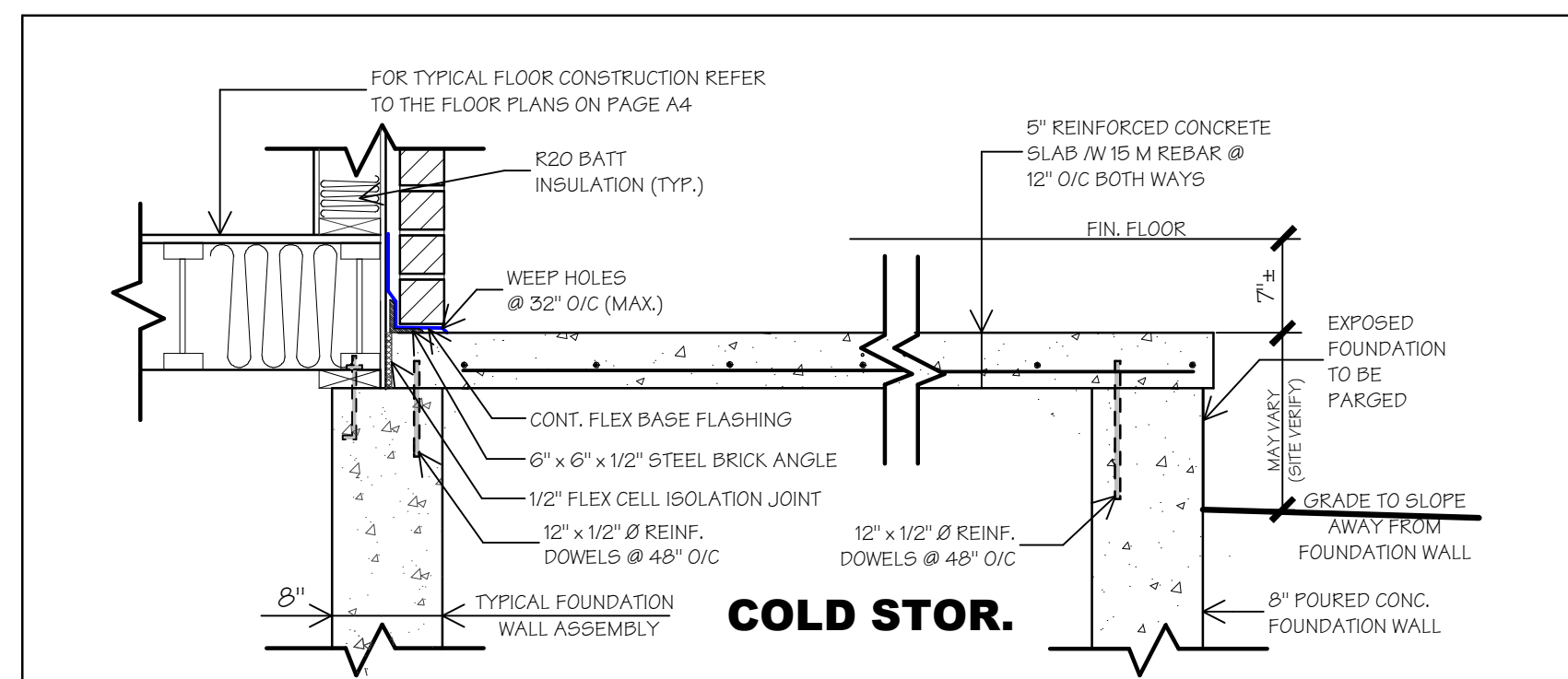
TYP. PORCH SLAB DETAIL SCALE: 3/4" = 1'-0"
