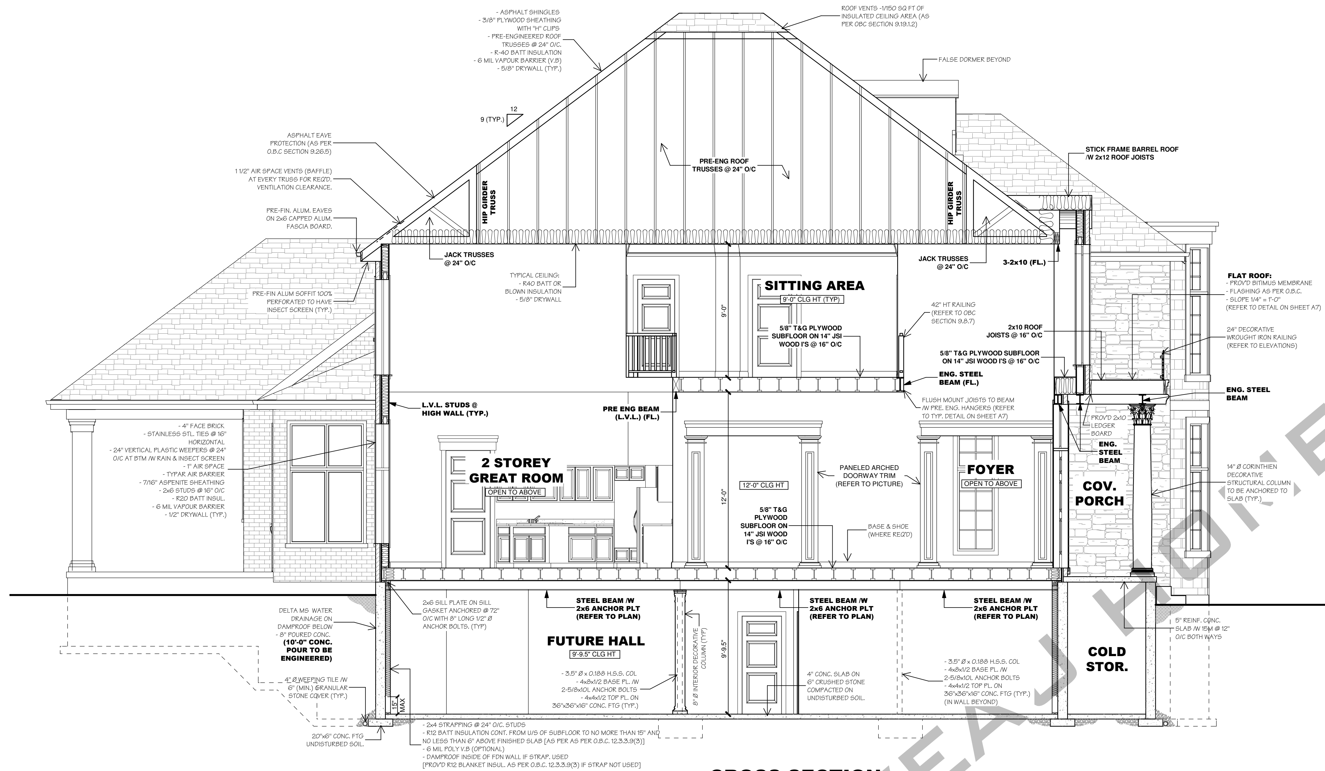
CROSS SECTION SCALE: 1/4" = 1'-0"
