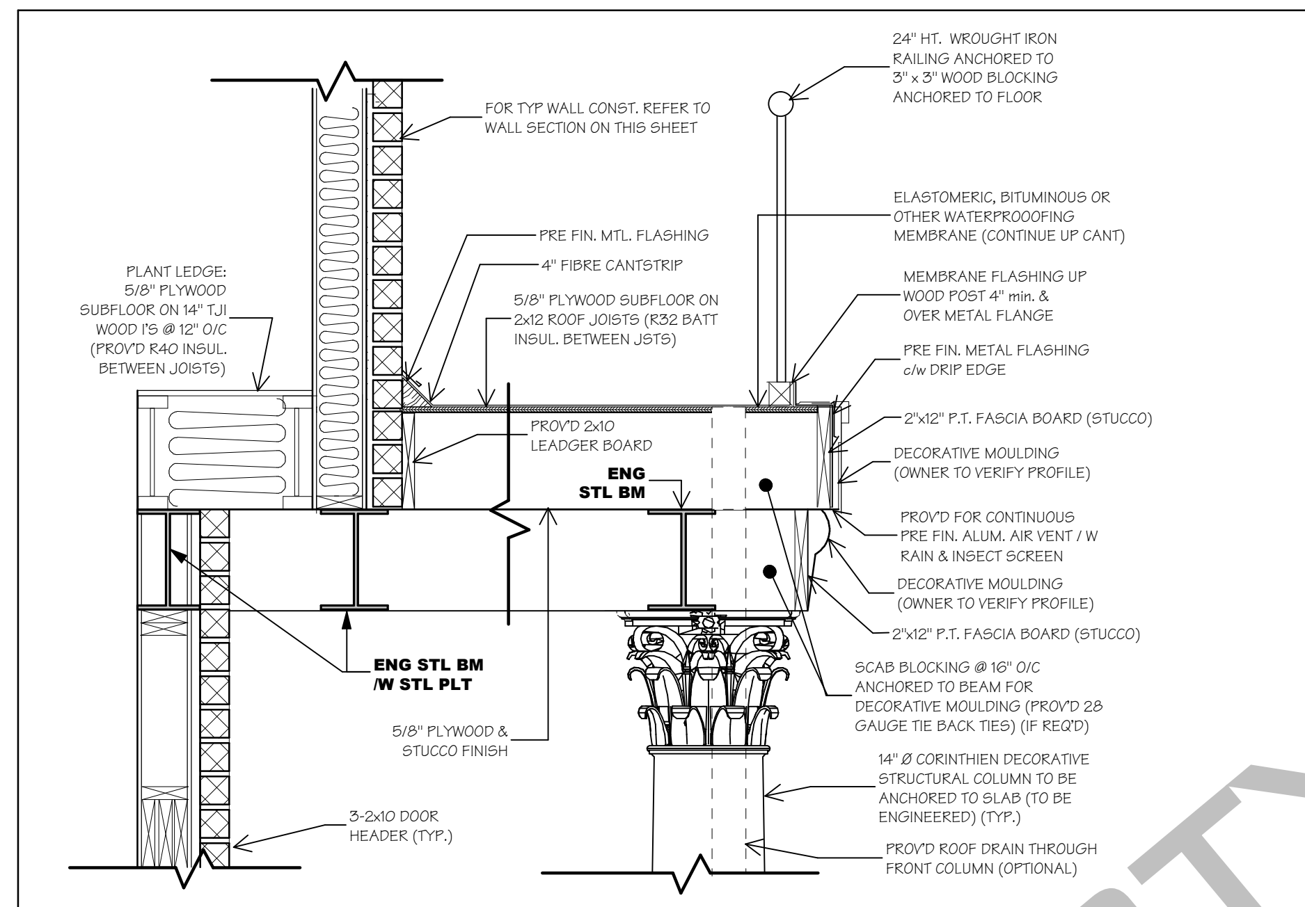
TYP. FLAT ROOF DETAIL SCALE: 3/4" = 1'-0"
